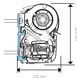
Montage mural consoles murales
